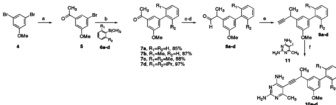
Scheme 2. Synthesis of Meta-Linked Biphenyl Inhibitors a
