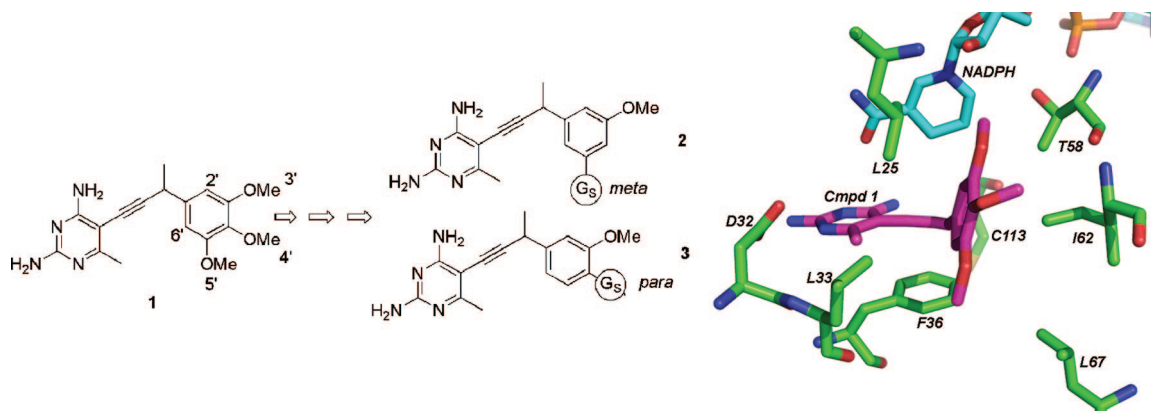
Scheme 1. Overall Strategy for Adding Steric Substitutions to the Meta or Para Position of the Initial Lead Compound a
